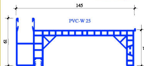
PROLONGADOR MOSQUITERA PROLONGER FOR MOSQUITO SCREEN TAPÉE MOUSTIQUEAIRE
