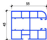
GUIA PVC 55x45 GUIDE COULISSE
